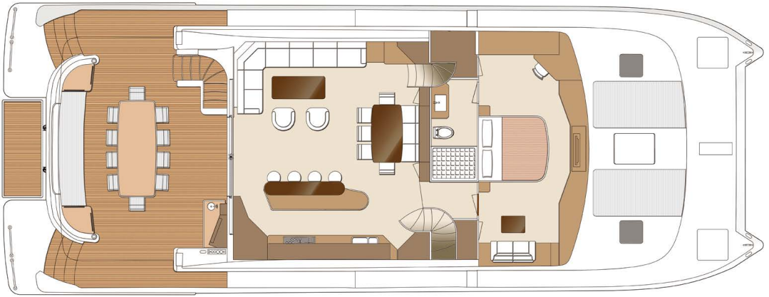
MAIN DECK
