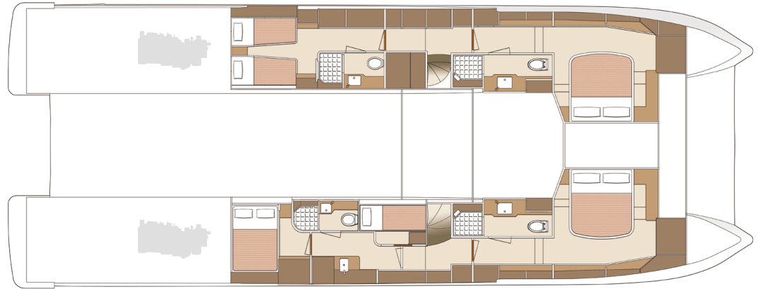
LOWER DECK
