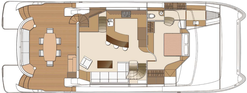
MAIN DECK
