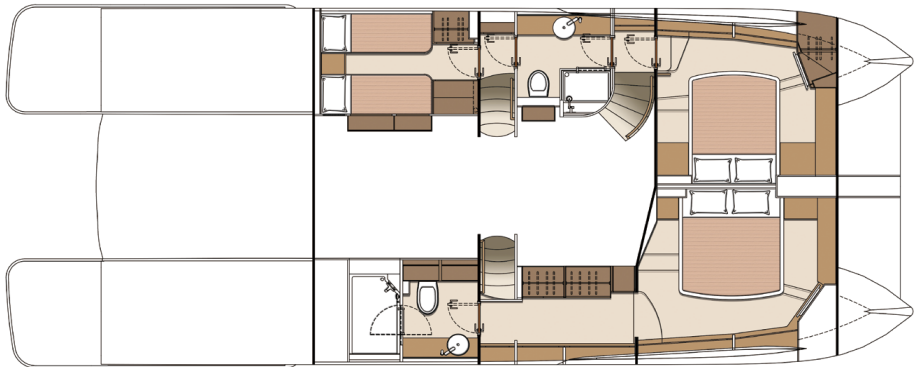
LOWER DECK
